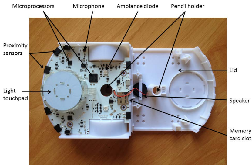
The motherboard, which holds the infrared sensors, central light touchpad, microprocessors and diodes
