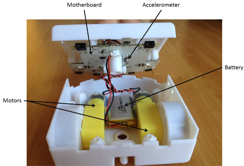
The chassis: the battery (in the middle) feeds the two motors (yellow) that turn the wheels
